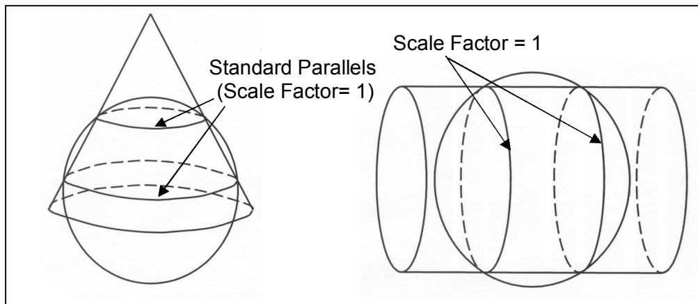
Figure 3. Conical (Lambert) and Cylindrical (Transverse Mercator) Map Projection Surfaces
