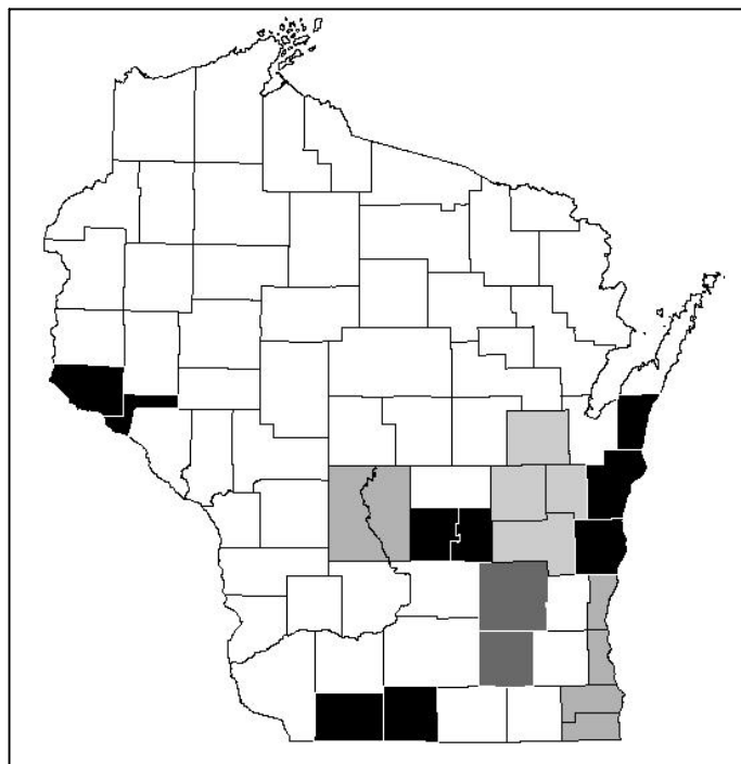
Figure 8. The Wisconsin County Coordinate System (Shaded Counties Share a Single System – There are 72 Counties and 59 Coordinate Systems (24 Lambert and 35 Transverse Mercator))
