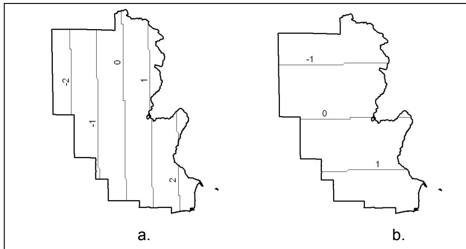
Isoline Maps of a) Easting (X) Shift and b) Northing (Y) Shift (in Millimeters) for Marinette County
