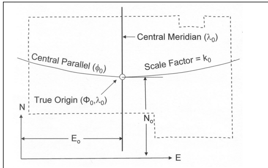
Figure 5. The Five Parameters of a Rectangular Coordinate System Based upon a Lambert Conformal Conical Projection
