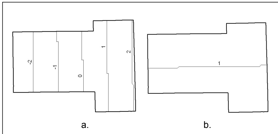
Isoline Maps of a) Easting (X) Shift and b) Northing (Y) Shift (in Millimeters) for Fond du Lac County
