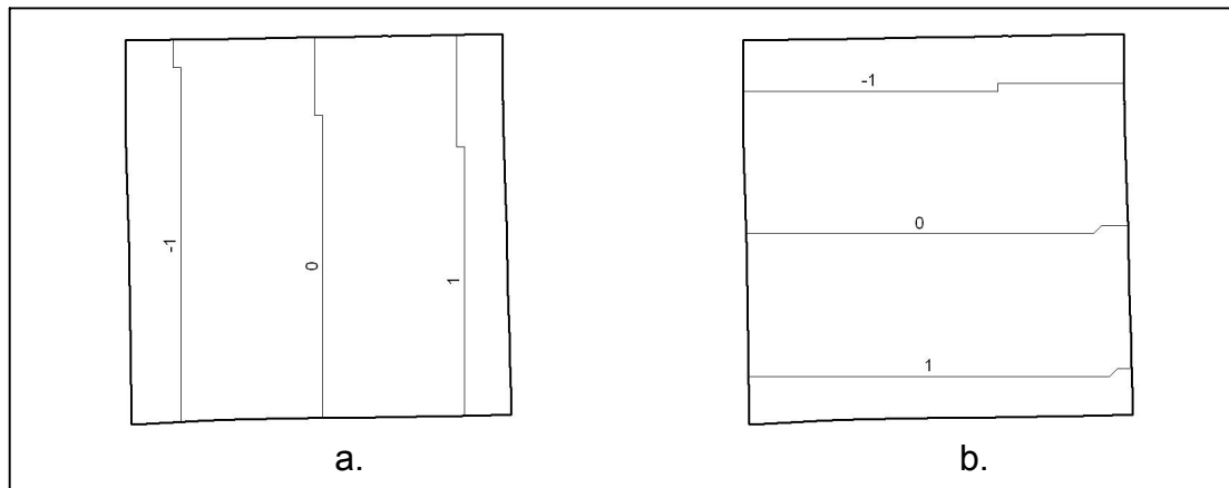
Isoline Maps of a) Easting (X) Shift and b) Northing (Y) Shift (in Millimeters) for Walworth County
