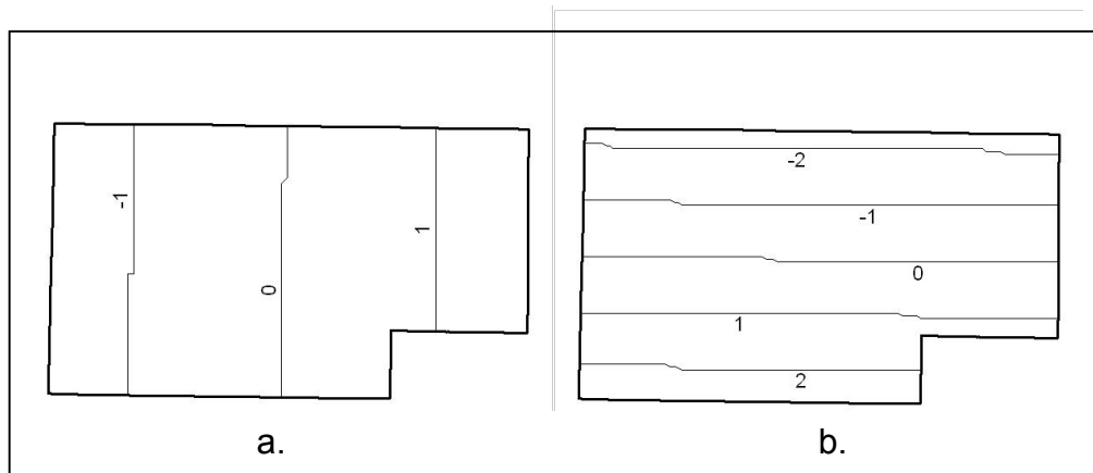
Isoline Maps of a) Easting (X) Shift and b) Northing (Y) Shift (in Millimeters) for Rusk County
