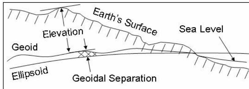
Figure 7. Elevation and Geoidal Separation
